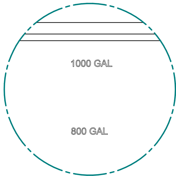
DETAIL B Typical Tank Markings and Graduation
